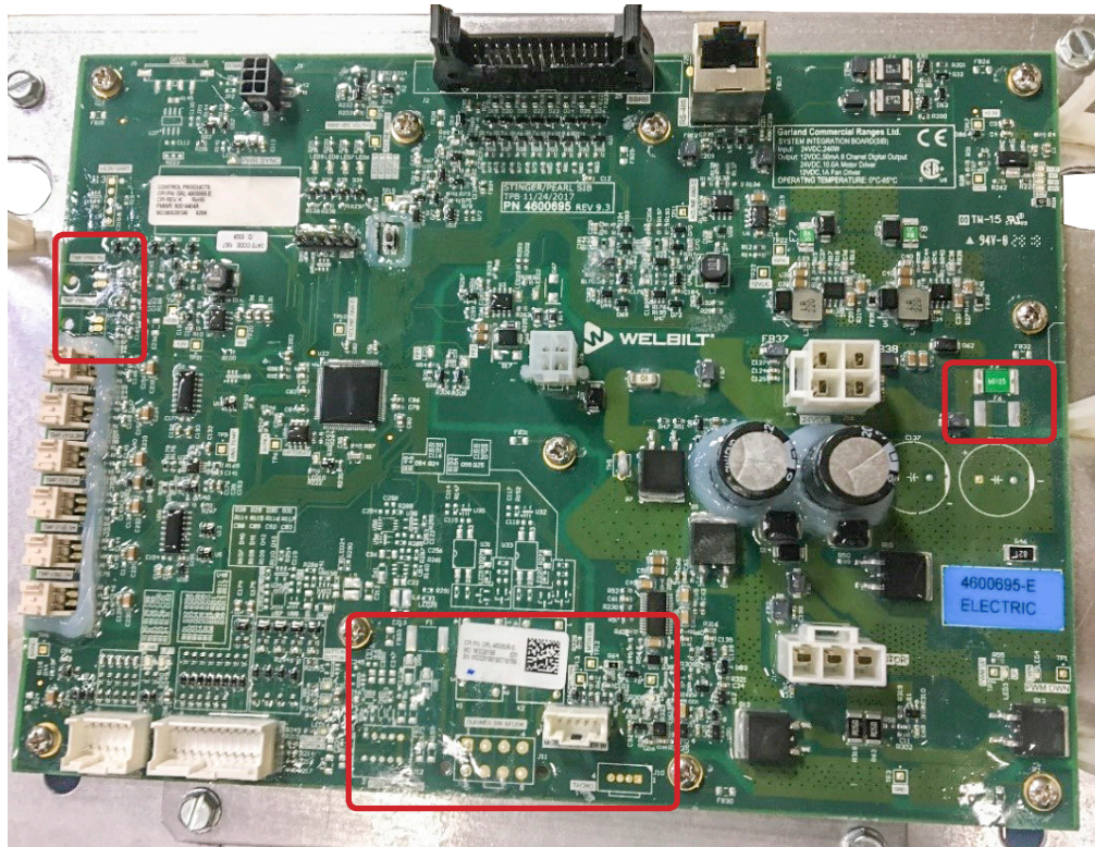
SIB Board (4600695-E) SIB ELCTRIC (ONLY SUITABLE FOR ELECTRIC UNITS)
