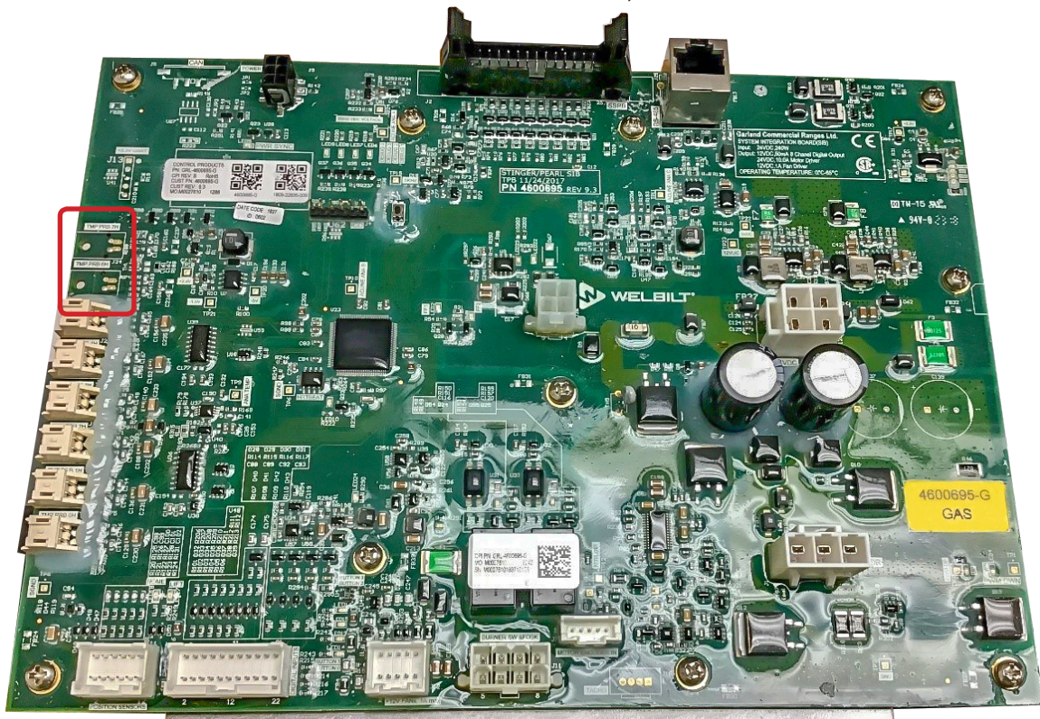
SIB Board (4600695-G) SIB GAS (SUITABLE FOR ALL UNITS AND WILL BE USED AS REPLACMENT PART)
